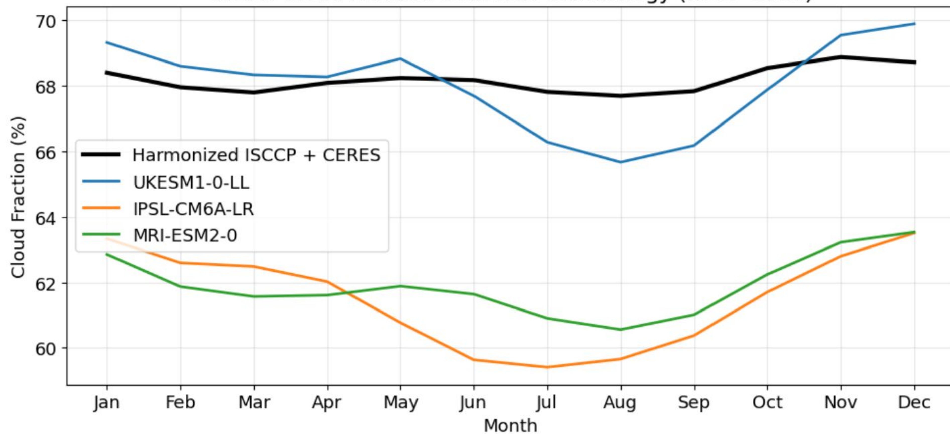
Global Cloud Fraction Seasonal Climatology (1983–2025)
