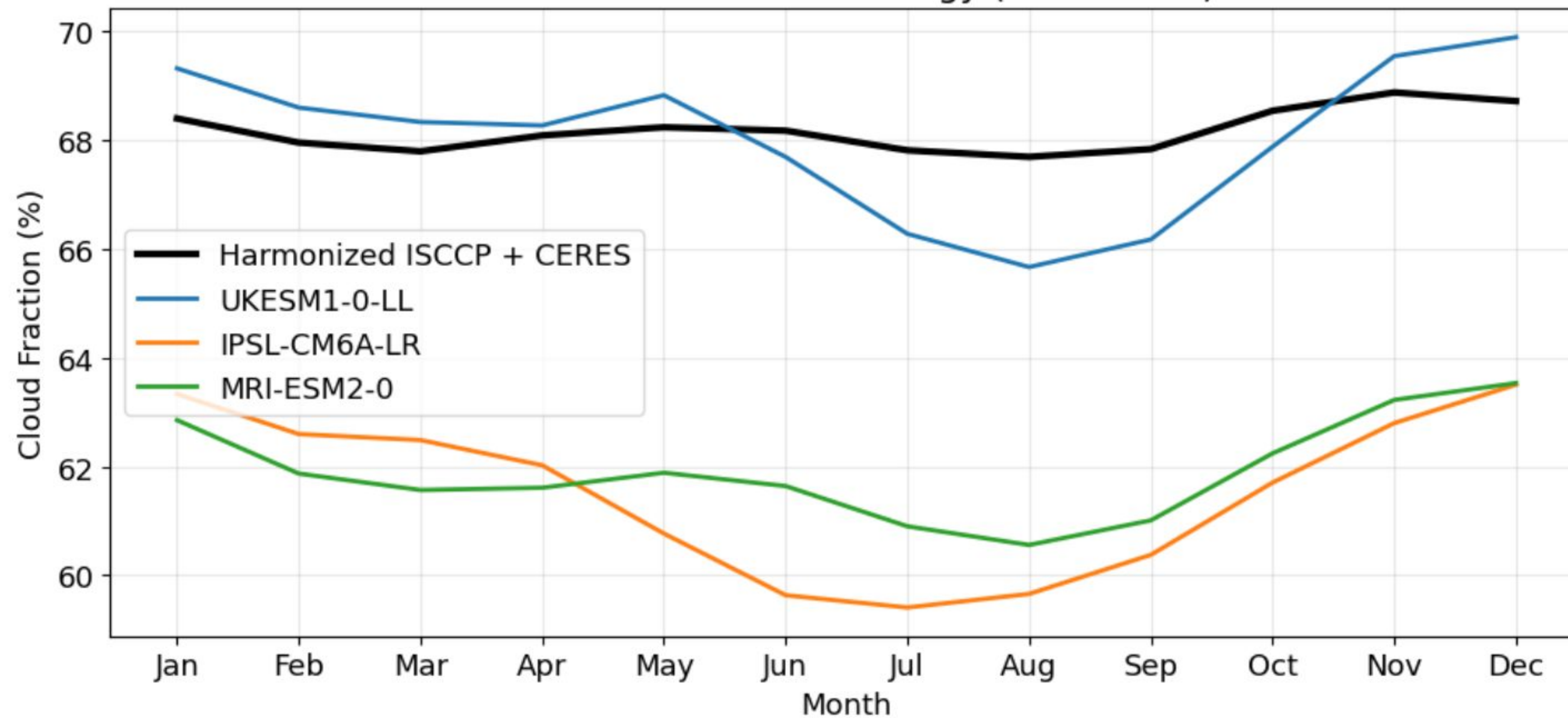
Global Seasonal Climatology (1983-2025)
