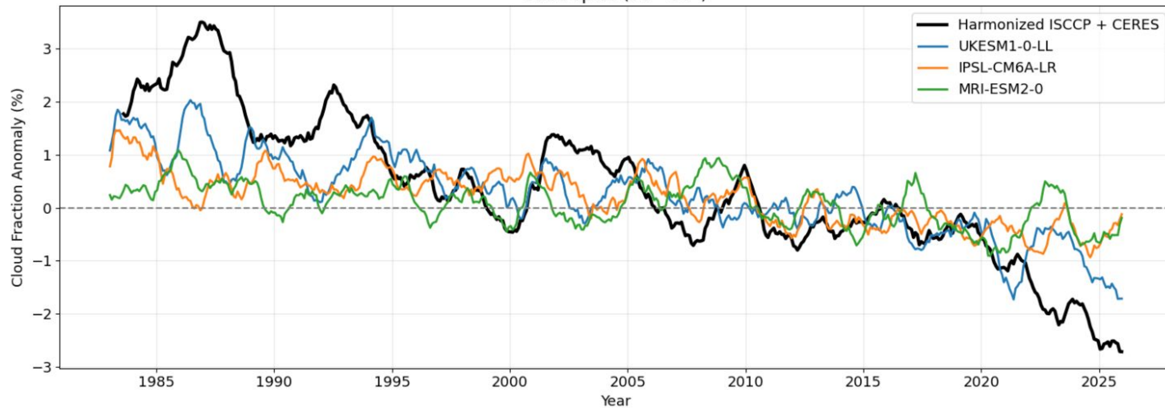
Cloud Fraction Anomalies (12-month Running Mean) Subtropics (30°-60°)
