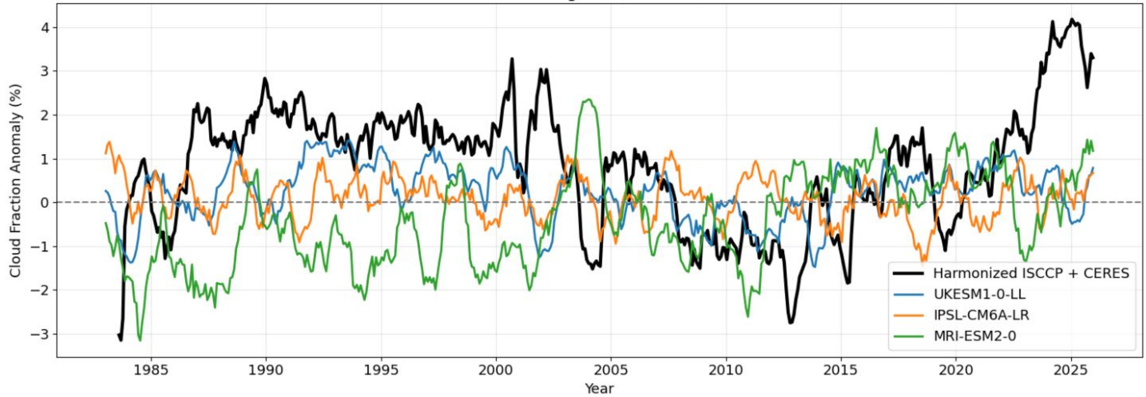
Cloud Fraction Anomalies (12-month Running Mean) Polar Regions (60°-90°)
