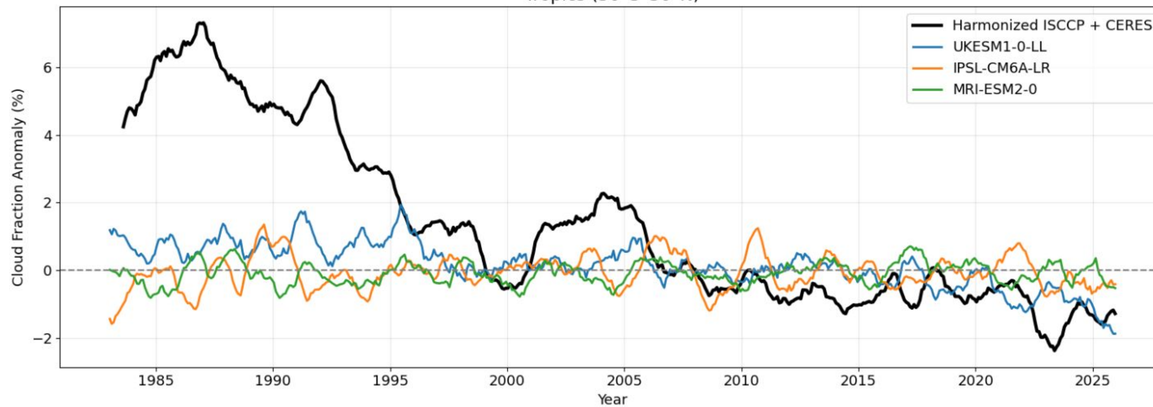
Cloud Fraction Anomalies (12-month Running Mean) Tropics (30°S-30°N)
