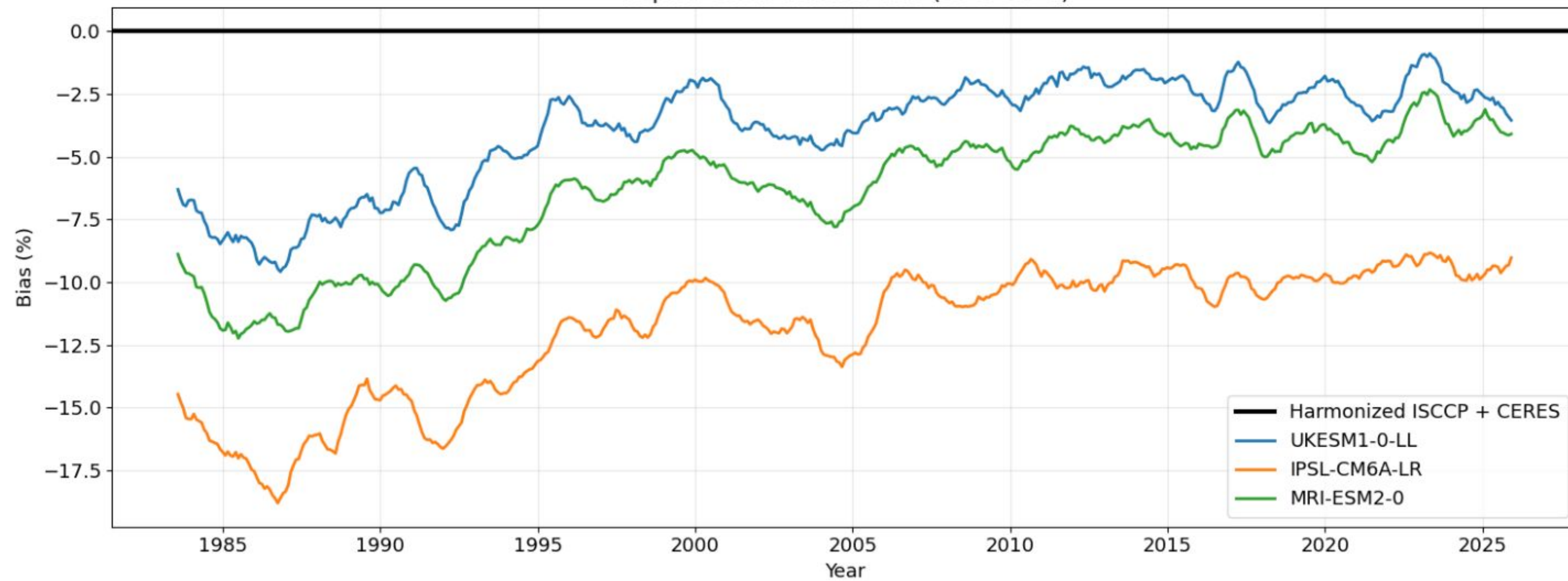
Tropical Cloud Fraction Bias (30°S-30°N)
